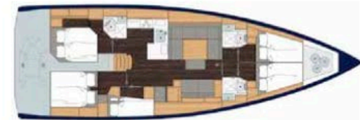
5-KABINEN-VERSION (A1-B2-C1-D2-E2) 5-CABIN VERSION (A1-B2-C1-D2-E2)
