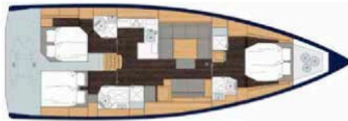
3-KABINEN-VERSION (A1-B1-C1-D1-E2) 3-CABIN VERSION (A1-B1-C1-D1-E2)
